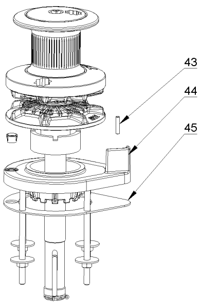
VW10 Arrangement
