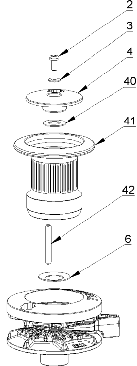
Capstan Arrangement
