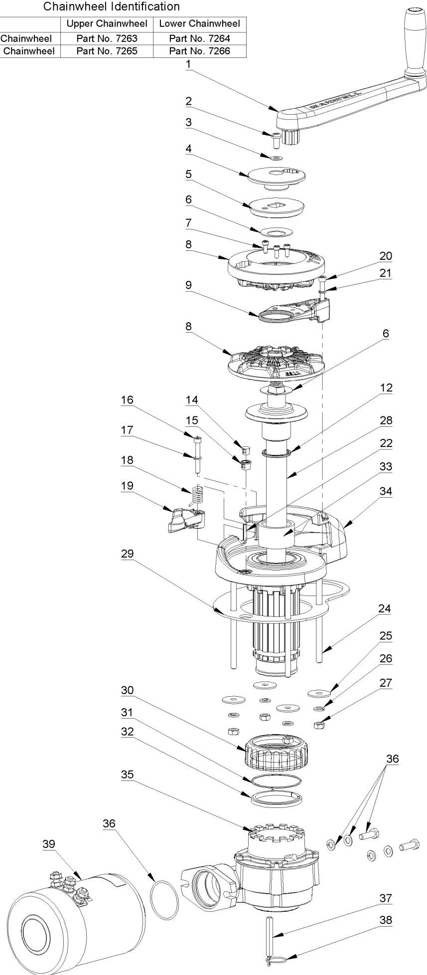
Capstan Arrangement
